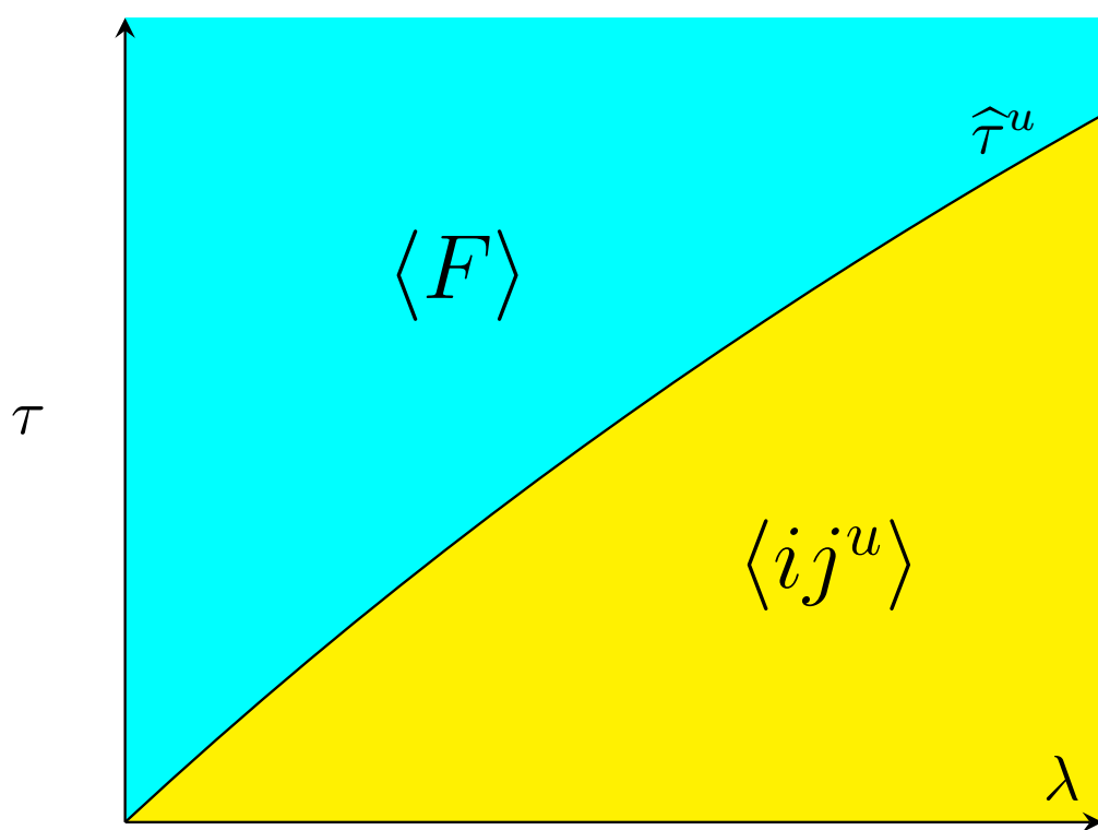
Figure 8: Stable equilibrium under CU - (CU game) Symmetry
